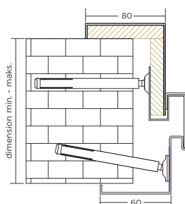
adjustable door frame PU-PR with coupling profile
