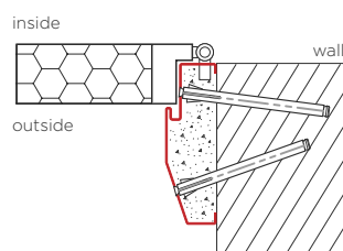
Assembly of the door frame PD56 on the inside of the wall
