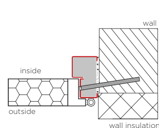
Assembly of the door frame Termo ODS on the outside of the wall
