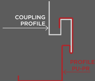
ADJUSTABLE FRAMES PU-PR WITH COUPLING PROFILE
