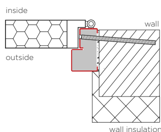
Assembly of the door frame Termo ODS on the inside of the wall
